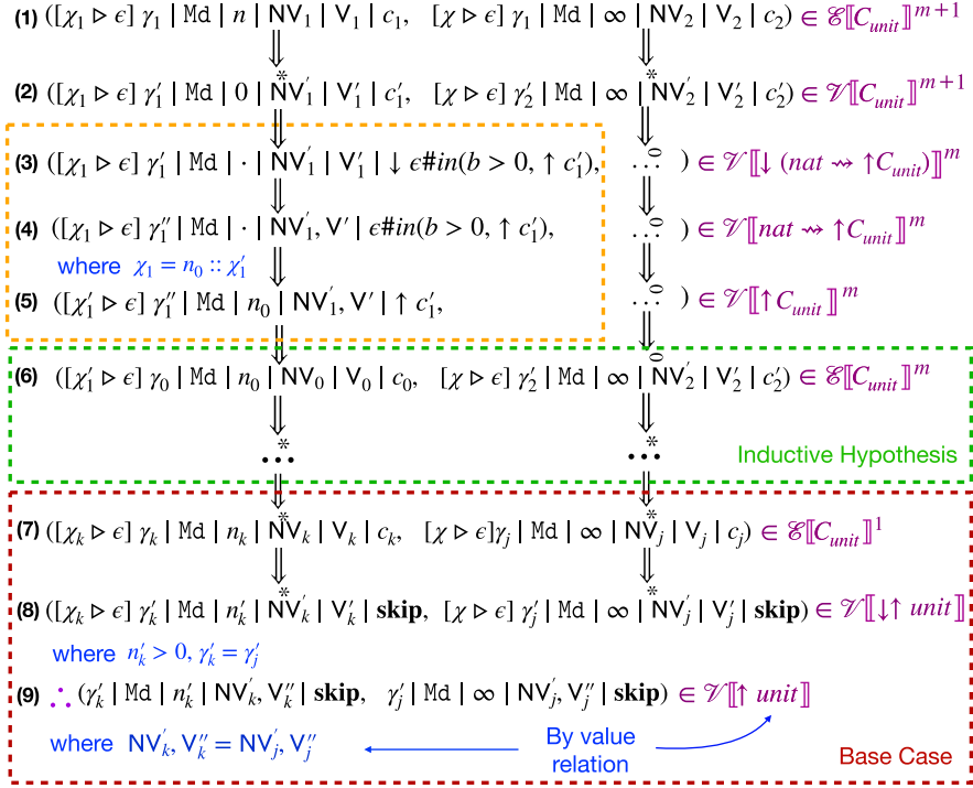
Fig. 28. Illustration of related configurations evaluating to the same store. We include the trace of the intermittent execution (left) and build the corresponding continuous execution (right). The purple text shows the relation between the two configurations at each step according to our logical relation. The orange box highlights the steps taken during a power failure. The green box highlights where the inductive hypothesis is applied. The red box highlights the base case. The blue text gives conditions that are known by assumption or are learned during the proof.
