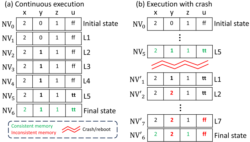
Fig. 2. An example execution of a1 with WAR dependencies with no variables checkpointed . NV denotes the nonvolatile memory. The subscript i indicates the memory after executing Line i .
